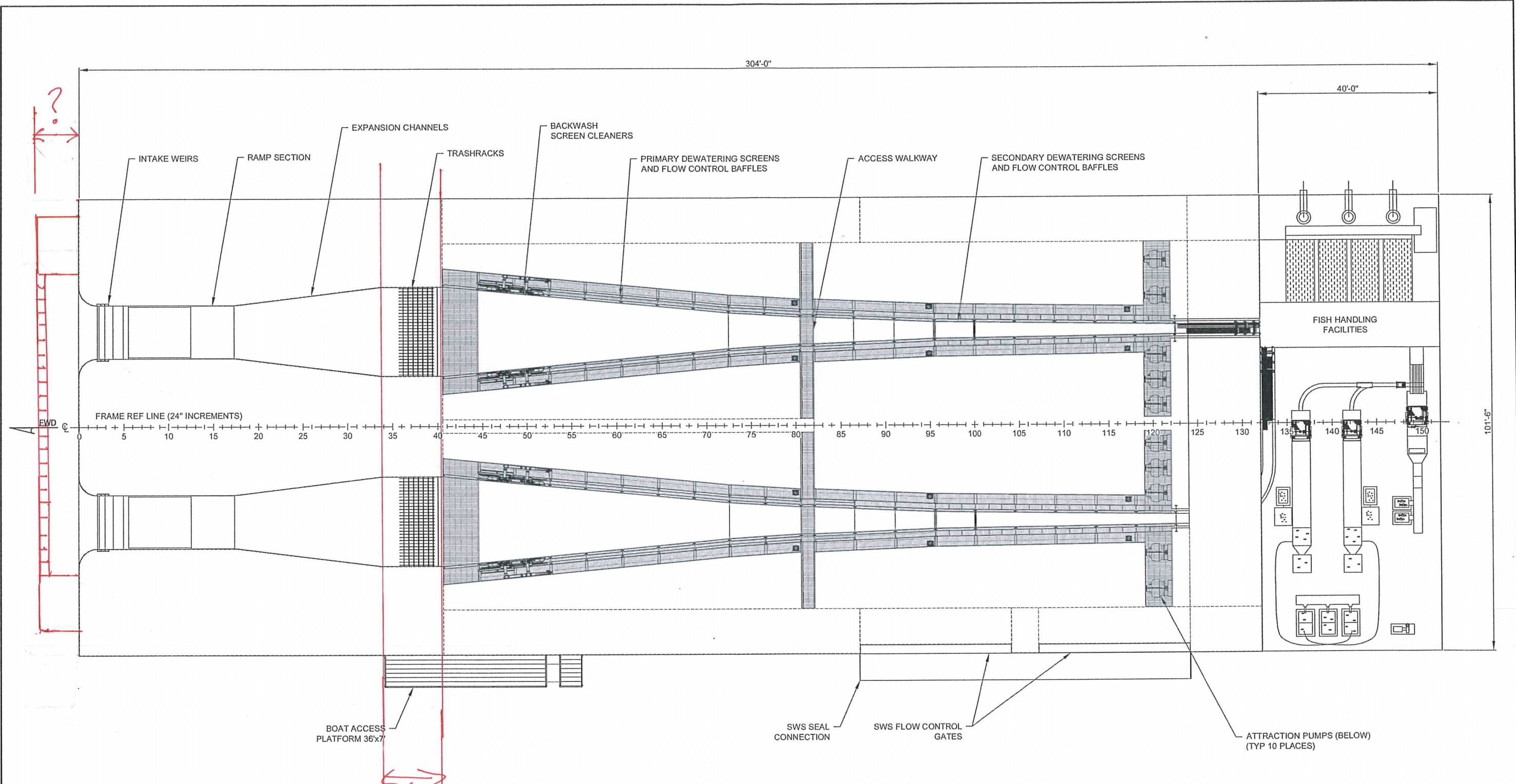
GENERAL ARRANGEMENT- MAIN DECK SCALE: 3/32" = 1'-0"
